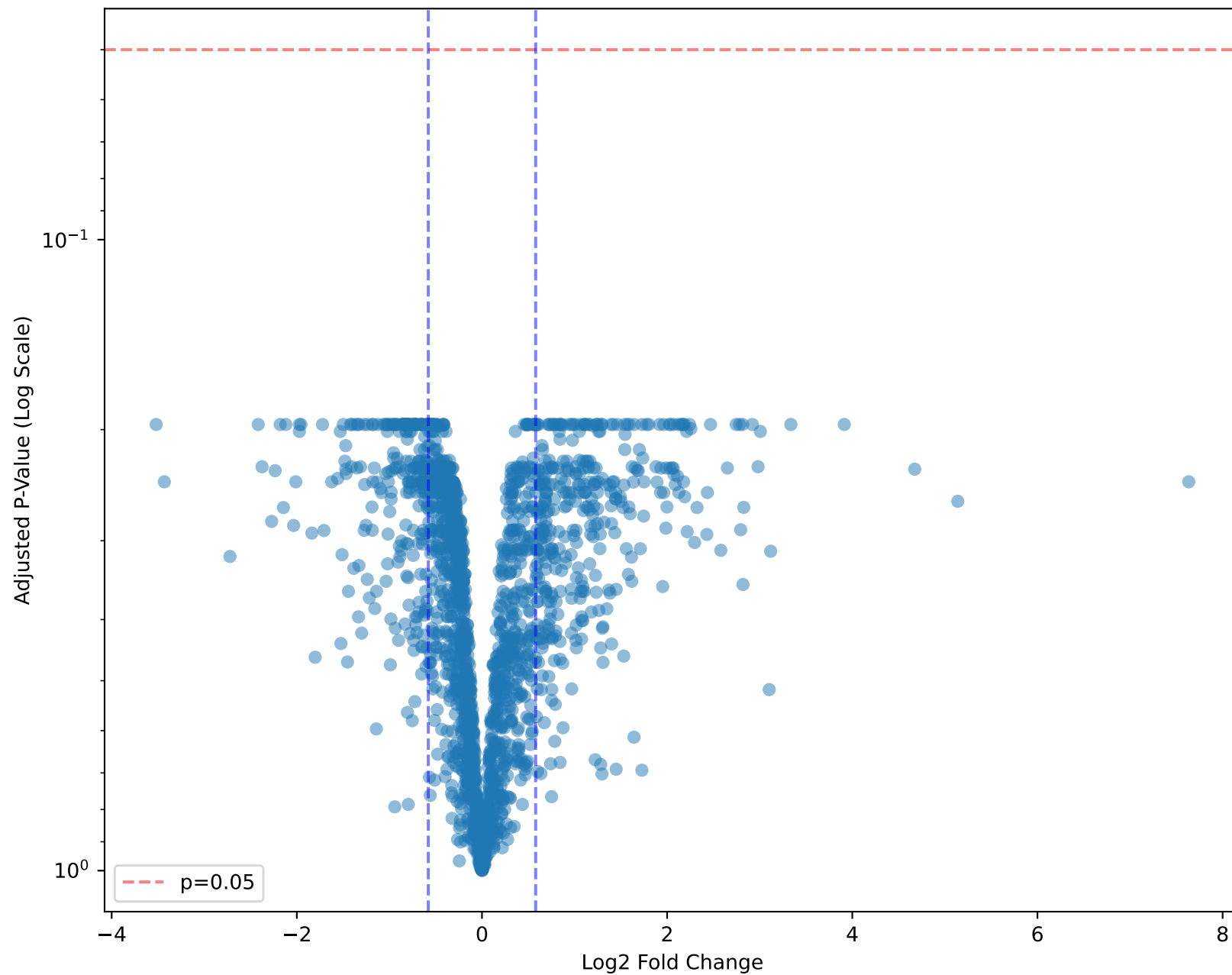
Volcano Plot: D9 - T0
